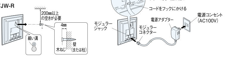
WJW-R
