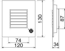
WJW-R
